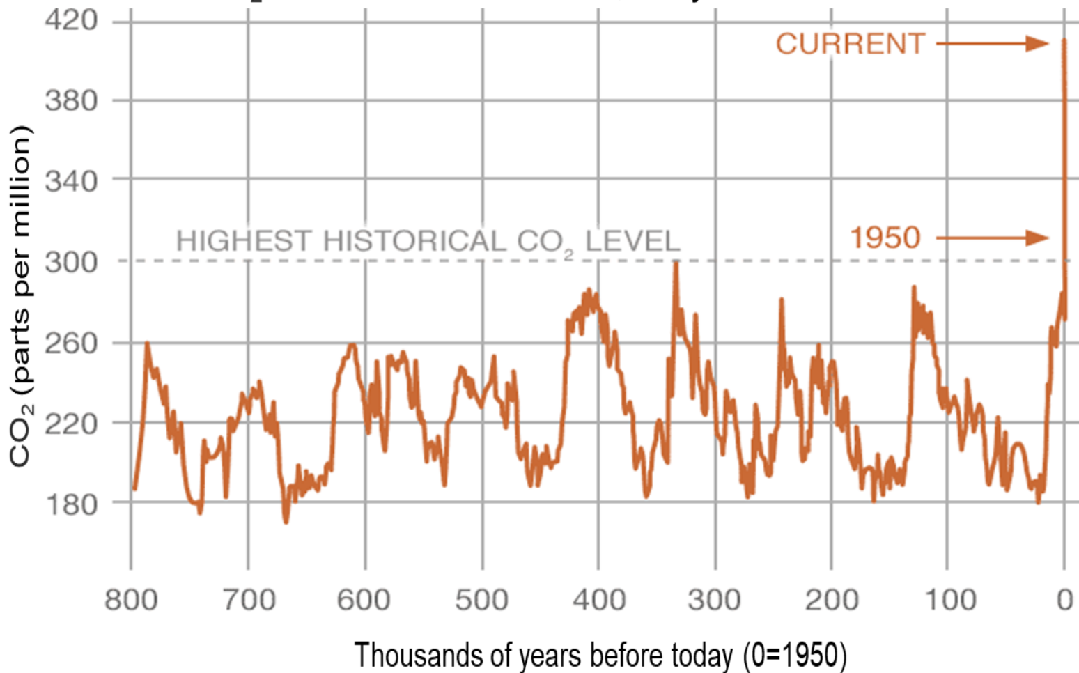
Global CO 2 levels over the last 800,000 years from ice core data
