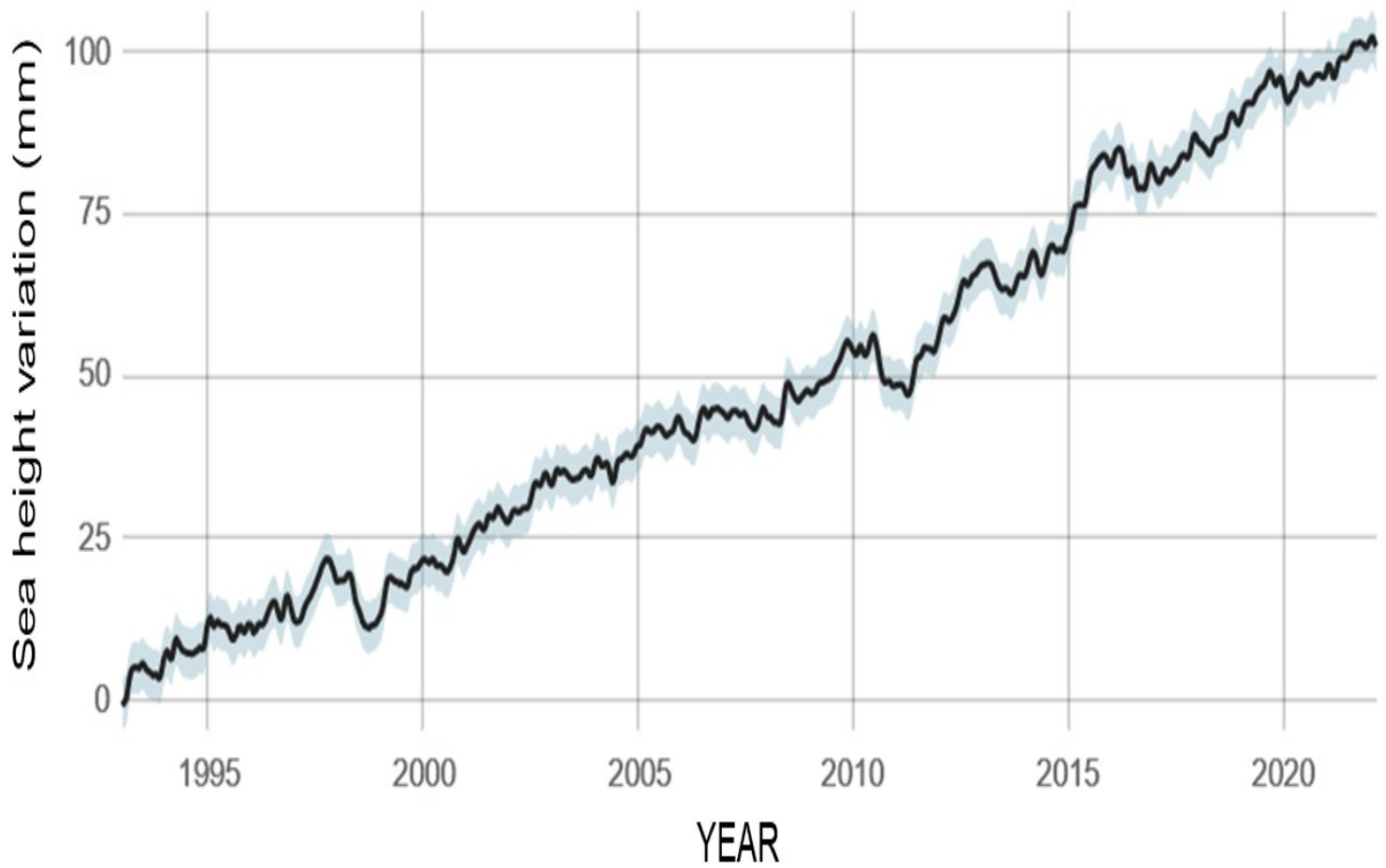
A graph showing global sea level rise since 1995 from satellite data
