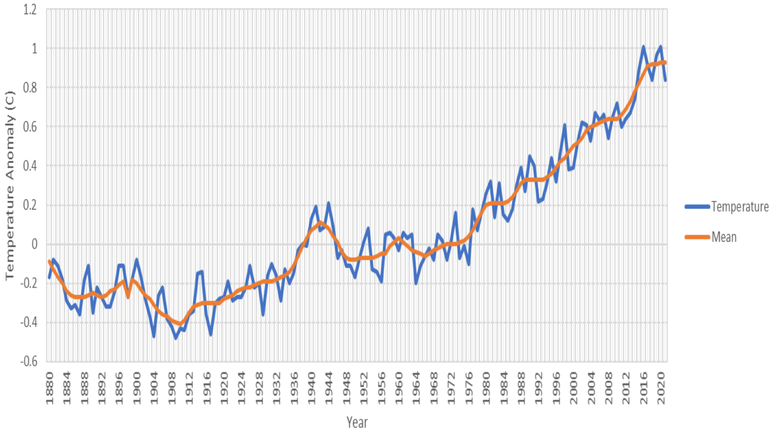
Graph showing change in global surface temperature from 1880-2020 relative to 1951-1980 average from temperature monitoring data
