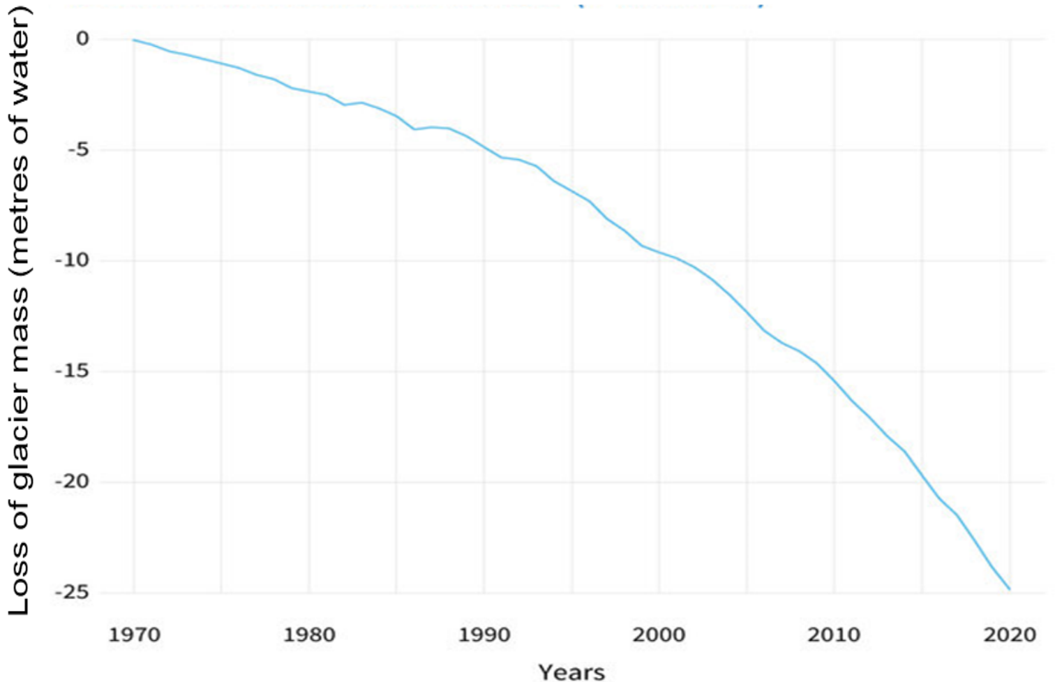
Graph to show ice lost from glaciers from glacier monitoring data
